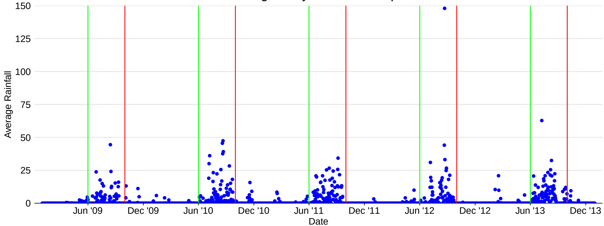
Average Daily Rainfall in Jaipur
